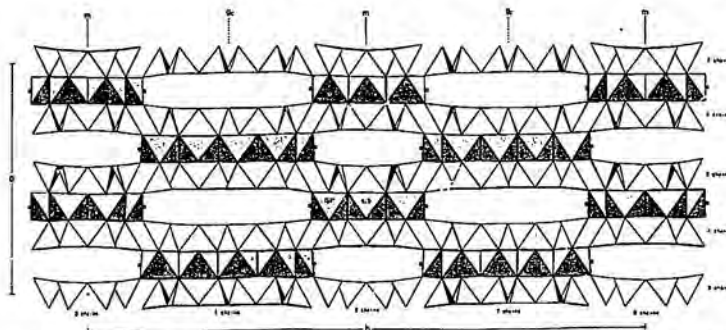
Fig. 10. (001) projection of the chesterite structure. The stacking sequence is ++-- and I-beams with double and triple chains alternate in the b direction. Double and triple B-chains are sandwiched between octahedral layers of like skew, while double and triple A-chains are between layers of opposite skew. Basal oxygen layers of all silicate chains are warped out of the (100) plane.
