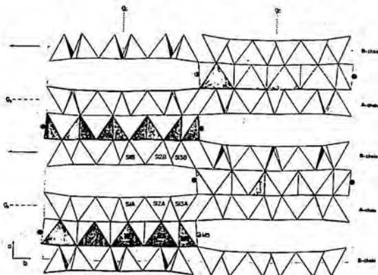
Fig. 4. Jimthompsonite structure projected onto (001). The stacking sequence is + + - -. B-chains occur between octahedral layers of like skew, while A-chains are between layers of opposite skew. The basal oxygen layers of the silicate chains are warped out of the (100) plane. The c -glide and b -glide are labeled "c" and "b." M5 is indicated by solid circles, and the unit cell is outlined.
