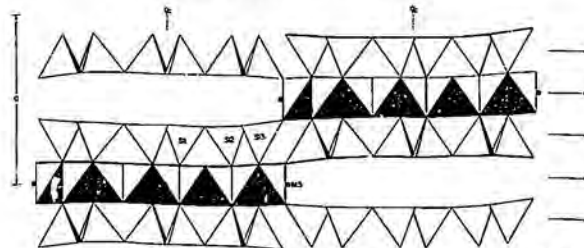
Fig. 6. c -axis projection of the clinojimthompsonite structure. The stacking sequence is + + +, and all triple chains are symmetrically equivalent. As in jimthompsonite, the basal oxygen layers of the silicate chains are warped out of the (100) plane.
